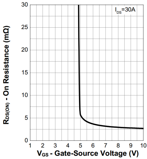
7. Transfer Characteristics
