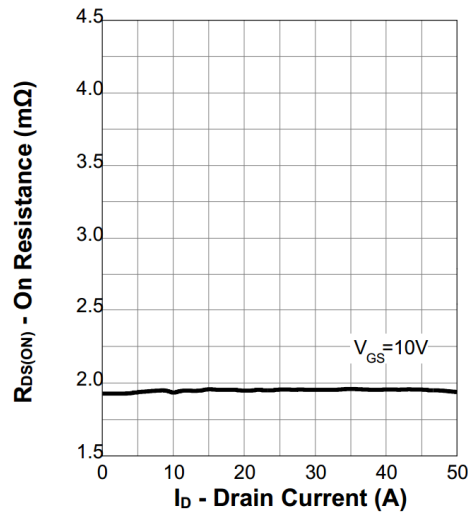
6. On Resistance
