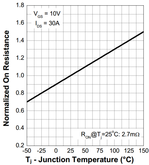
9. Normalized On Resistance
