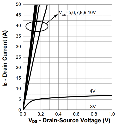
5. Output Characteristics
