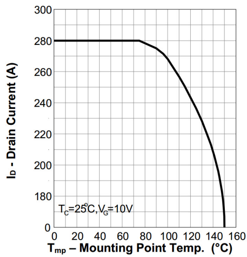
2. Current Capability
