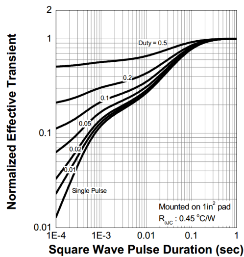
4. Transient Thermal Impedance
