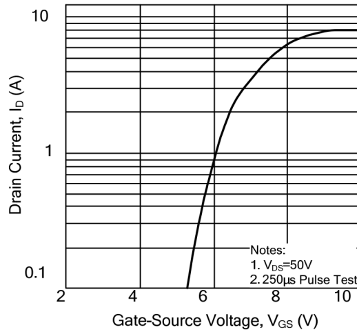
4. Transfer Characteristics
